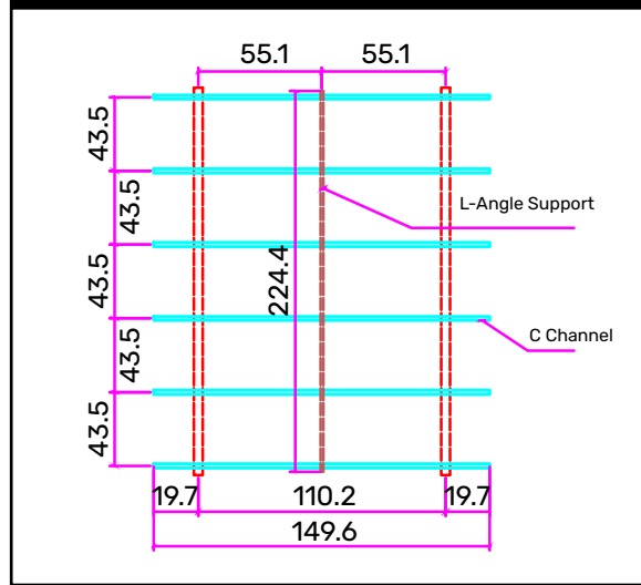
C-Channel Layout
