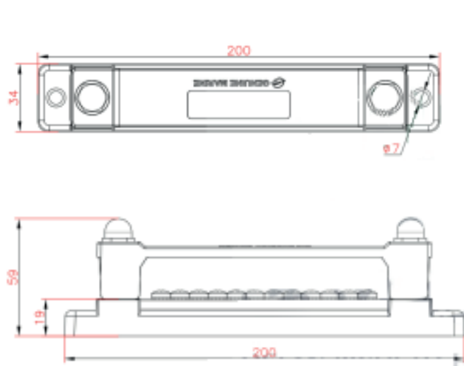
Busbar 300 A 2P with 12 screws and cover (05-052029-11 )
