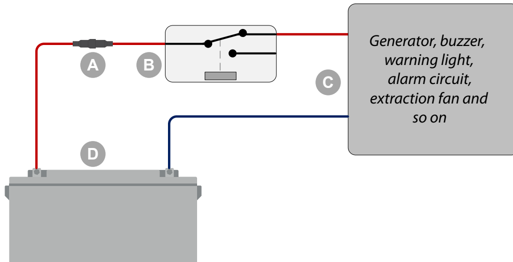
Figure 1. Programmable relay wired to operate a load
