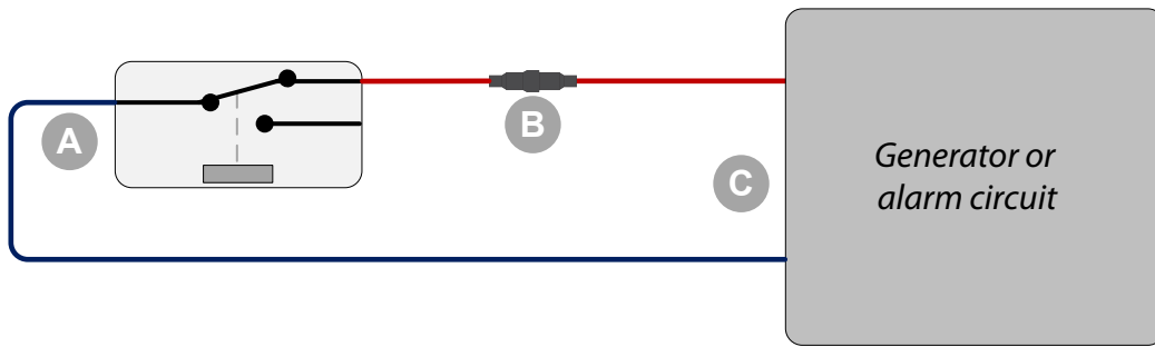
Figure 2. Programmable relay wired to operate as a potential free contact switch
